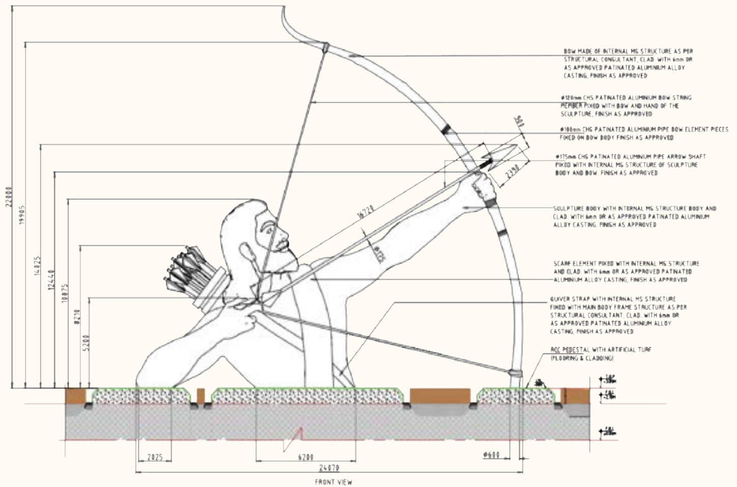
FRONT ELEVATION
